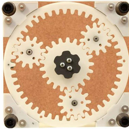
MEG-PNTY: Planetary Gear Set Model
