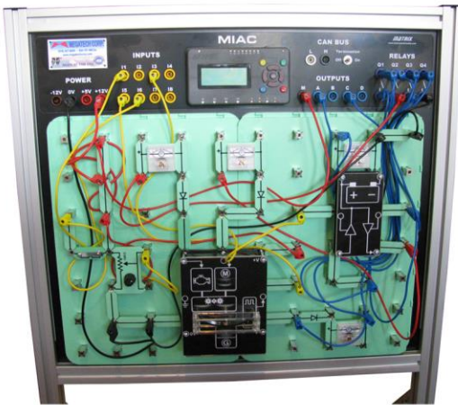
MEGLOC - HYBRID Hybrid Demonstrator Trainer
