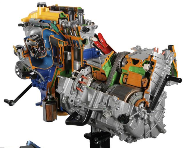
MEGART-PRIUS Prius Engine Cutaway
